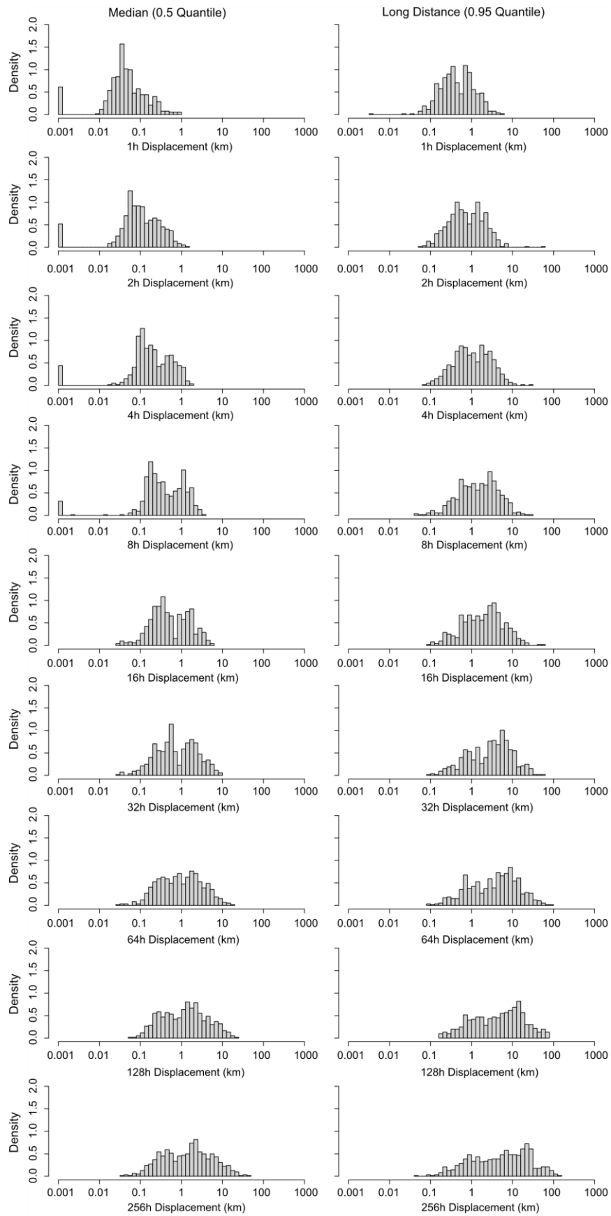
Fig. S1. Distributions of the median and 0.95 quantiles of the individual displacements used in the analyses. The y-axis represents the density distribution of median (0.5 quantile) and long-distance (0.95 quantile) displacements of each individual.
